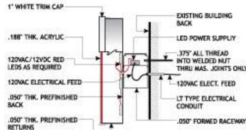
TYPICAL SECTION & DETAIL NOT TO SCALE
