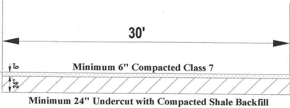
Typical Drive Cross-section
