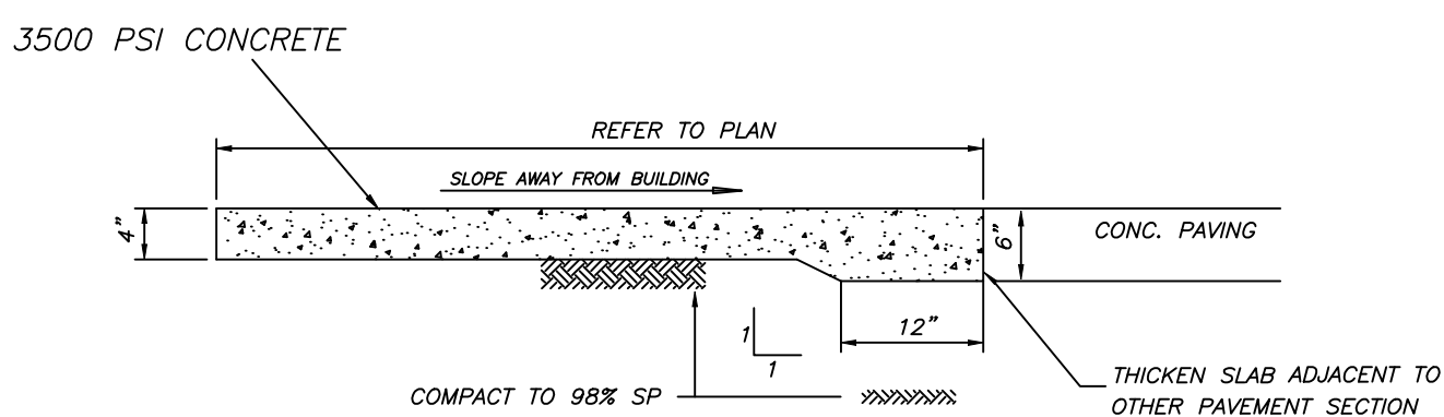
CONC. SIDEWALK – TYPE 'B' NTS
